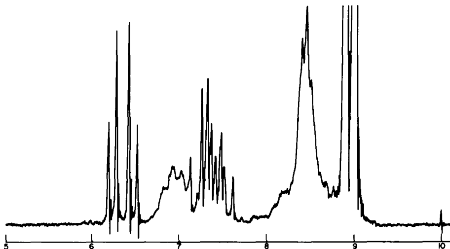
FIG. 6 NMR spectrum of trans -2,6-H-2-methyl-8-isopropyl 1,8-diazabicyclo[4.3.0]nonane.
