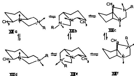
FIG. 2 Conformations of 8-alkyl cis -2,6-H-2-methyl-1,8-diazabicyclo[4.3.0]nonanes.
