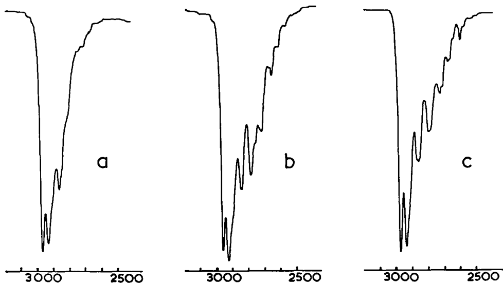
FIG. 4 C—H stretching region of IR spectra of: a. trans -2,6-H-2-methyl,8-t-butyl-1,8-diazabicyclo[4.3.0]nonane b. 8-t-butyl 1,8-diazabicyclo[4.3.0]nonane c. cis -2,6-H-2-methyl,8-t-butyl-1,8-diazabicyclo[4.3.0]nonane.
