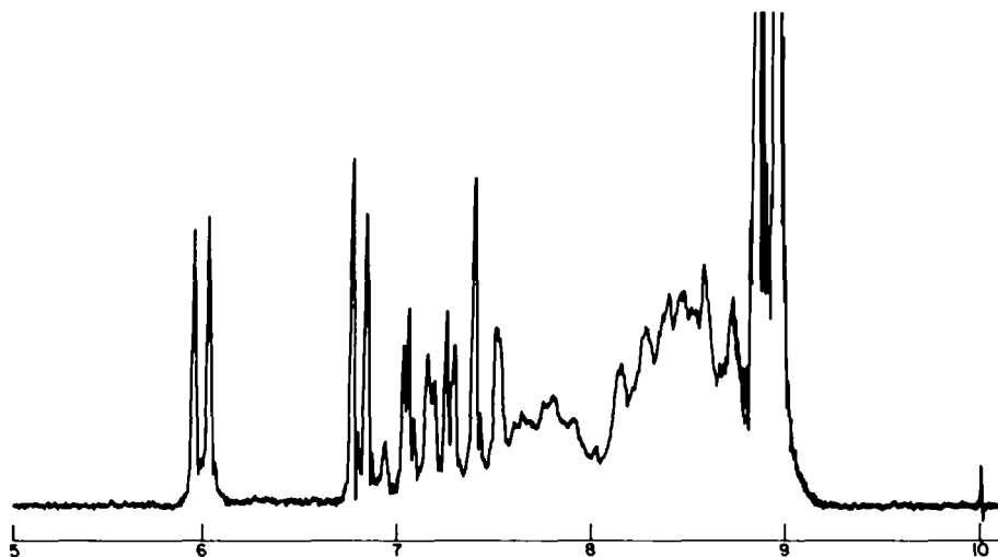
FIG. 5 NMR spectrum of cis -2,6-H-2-methyl-8-isopropyl 1,8-diazabicyclo[4.3.0]nonane.
