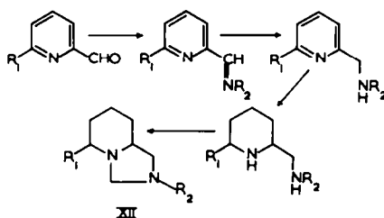
FIG. 1 Preparation of 8-alkyl-1,8-diazabicyclo[4.3.0]nonane.
