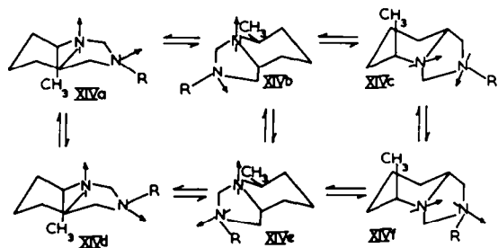
FIG. 3 Conformations of 8-alkyl trans -2,6-H-2-methyl-1,8-diazabicyclo[4.3.0]nonanes.
